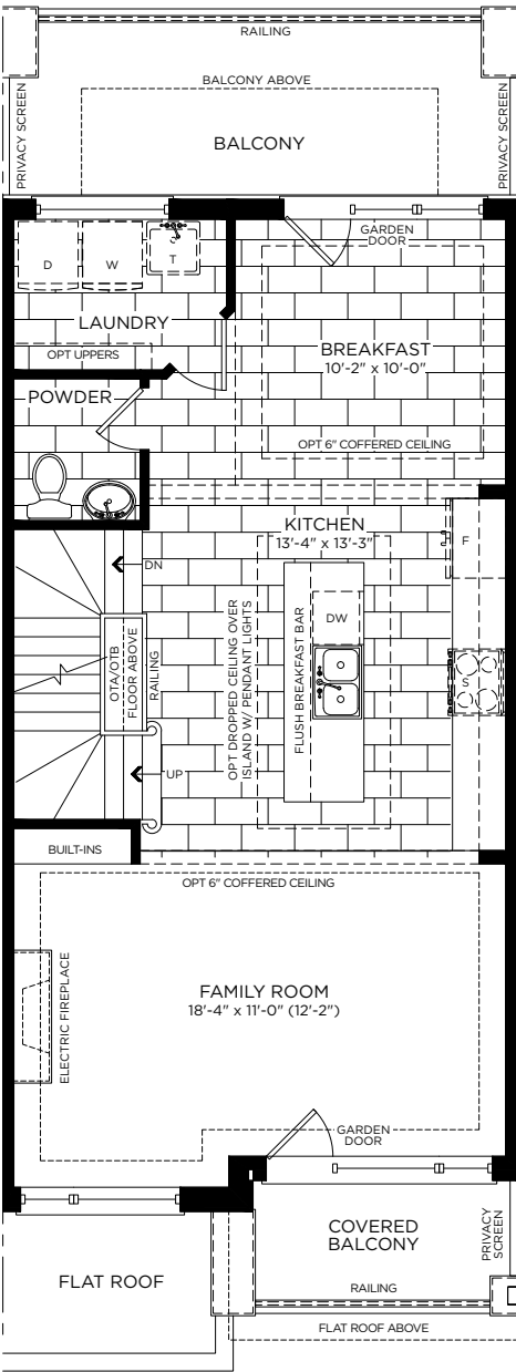
Main Floor
