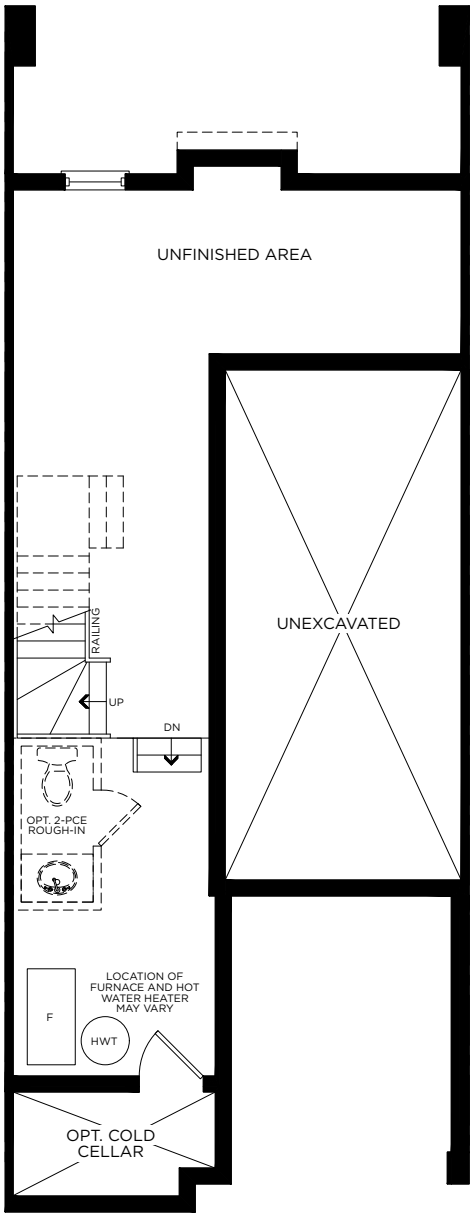
Basement
