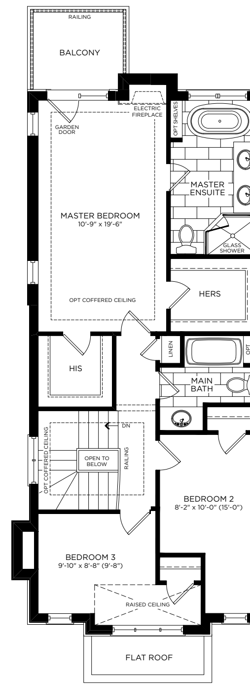
Upper Floor
